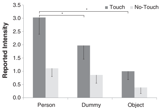
Fig. 1. Reported intensity of synaesthetic touch to the movie stimuli used in the fMRI study (from N = 9 mirror-touch synaesthetes). Error bars show 1 SEM. Horizontal lines indicate significant differences between touch conditions ( p < 0.05 ).
