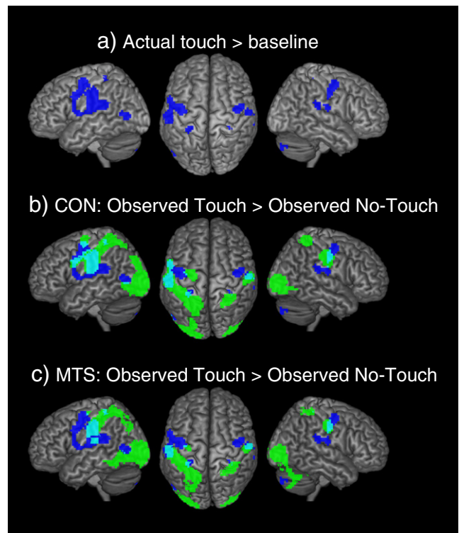
Fig. 2. (a) Results from the touch localiser shown in dark blue; (b) shows the contrast of observed touch vs observed no-touch (in green) as well as its conjunction (cyan) with actual touch in controls; (c) Observed touch vs. Observed no-touch (green) and its conjunction (cyan) with actual touch in MTS.
