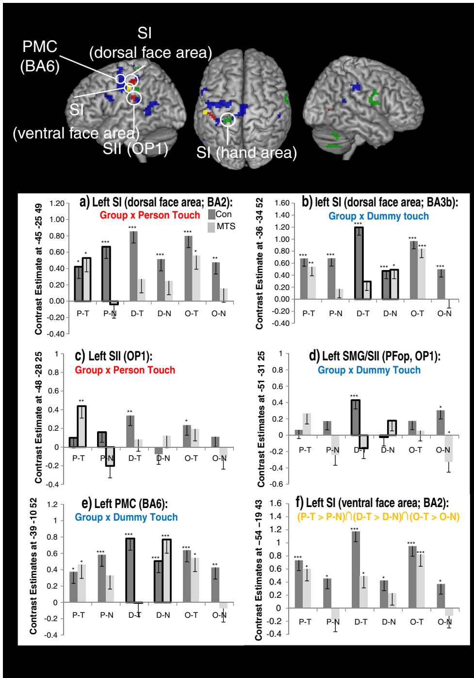
Fig. 3. Surface rendering of areas showing significant Group × Touch interactions. Areas marked in red, blue and green show a significant interaction of Group × Person Touch, Dummy Touch and Object touch, respectively. Yellow areas indicate significant activation for the conjunction (PT - PN) \cap (DT - DN) \cap (OT - ON) . a)–f) illustrate the interaction for selected key regions. Bar graphs for conditions that are relevant to the particular interaction shown are highlighted by thick black borders. Light grey bars indicate synaesthetes, dark grey bars indicate controls. Asterisks indicate whether the contrast estimate is significantly different from 0 (fixation baseline). Error bars show 1 SEM. * p < .05 , ** p < .01 , *** p < .005 .
