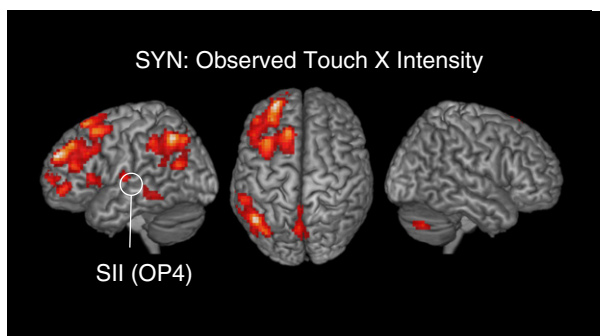
Fig. 4. Regions showing significant correlations between BOLD signal and intensity of synaesthetic touch (measured outside of the scanner) considering all types of stimuli.
