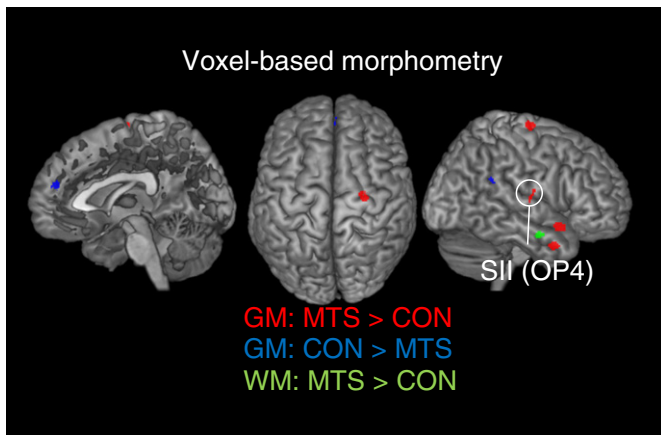
Fig. 5. Results of voxel-based morphometry analysis showing group differences in Grey Matter (GM) and White Matter (WM) volume.
